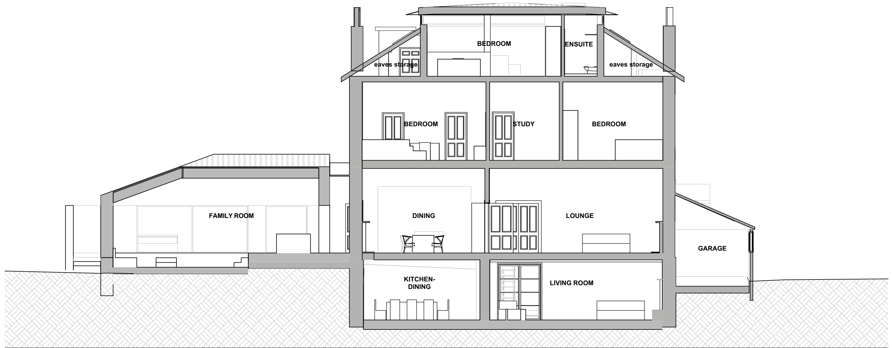
1 Section AA 1:100
