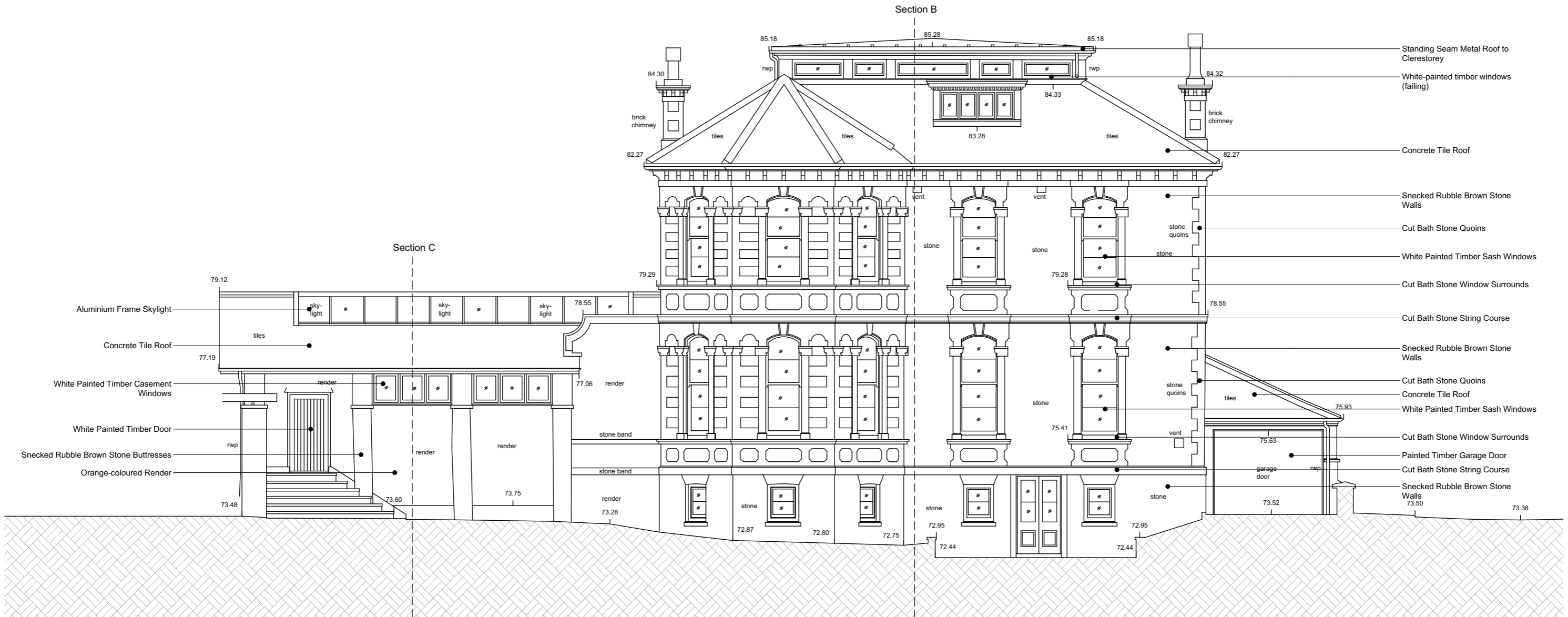
1 Front Elevation 1:100
