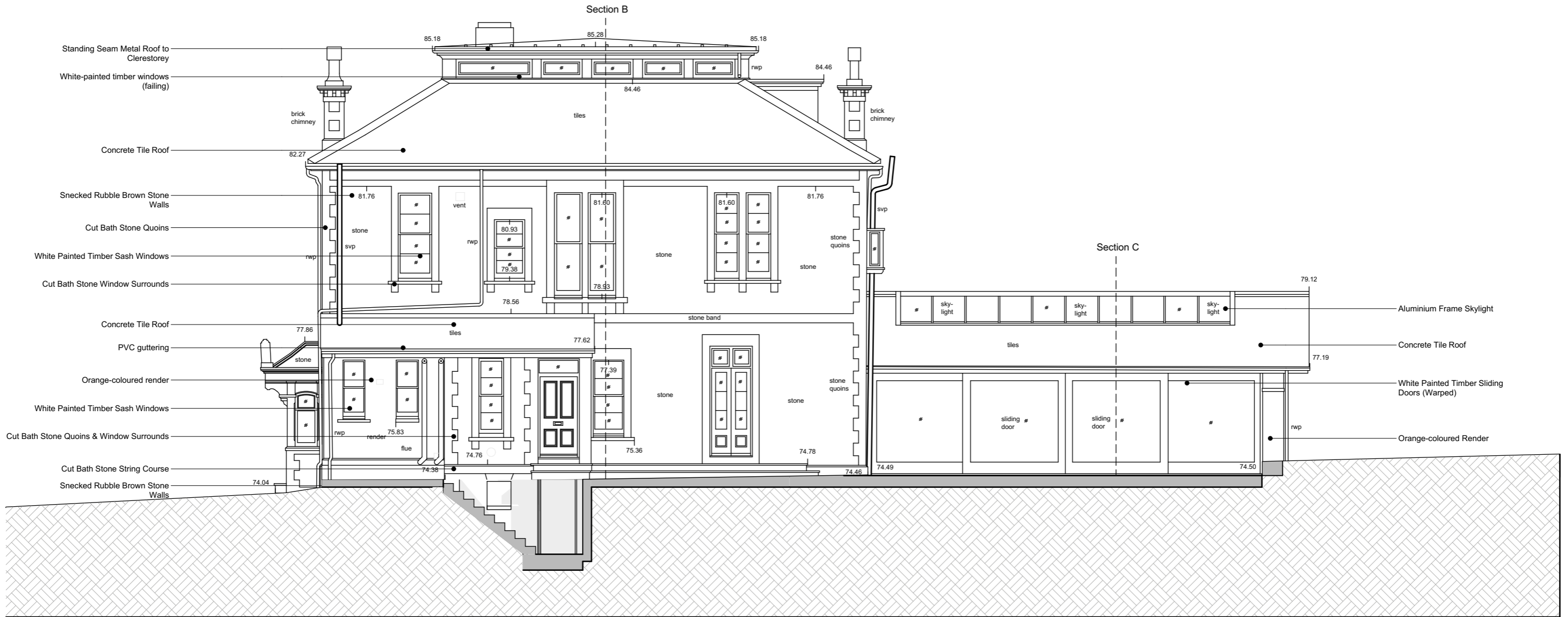
2 Rear Elevation 1:100
