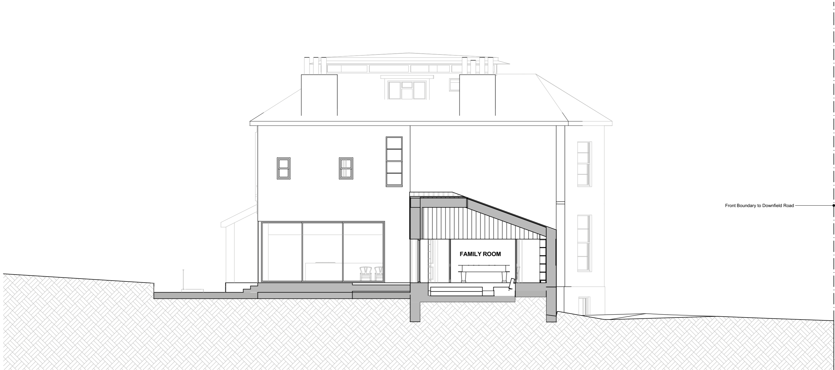
1 Section CC 1:100
