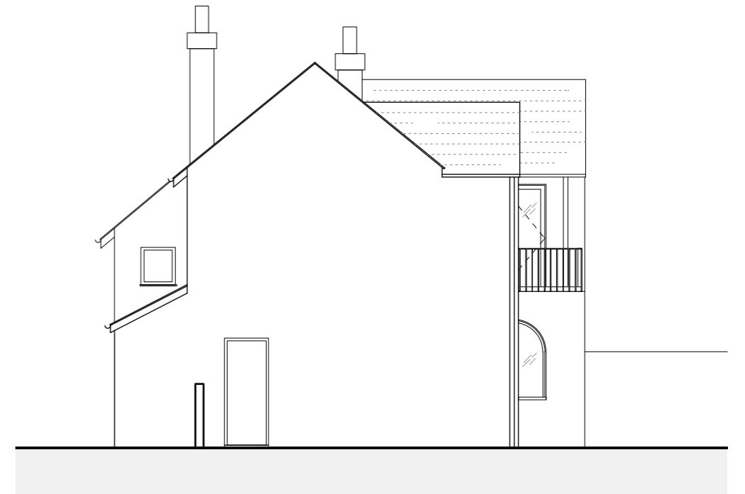
west elevation
