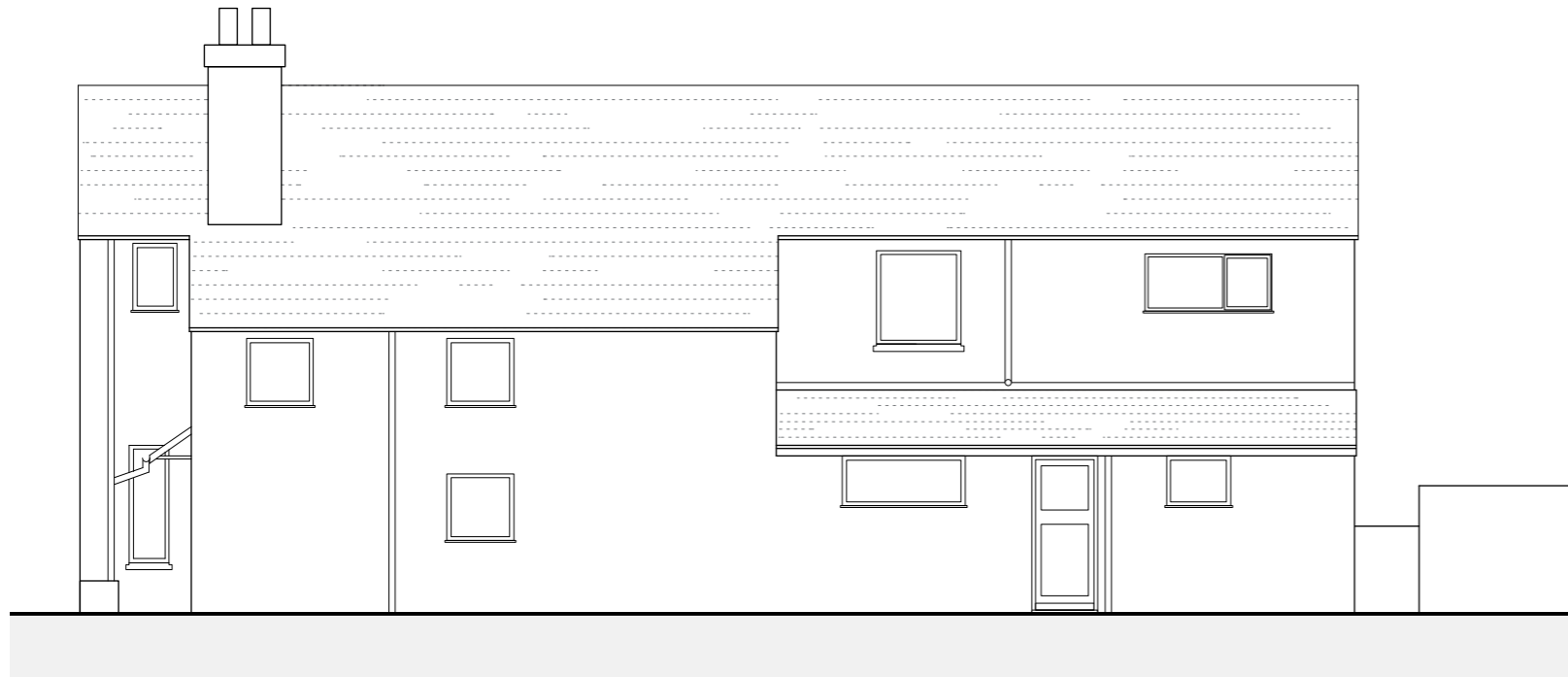
north elevation
