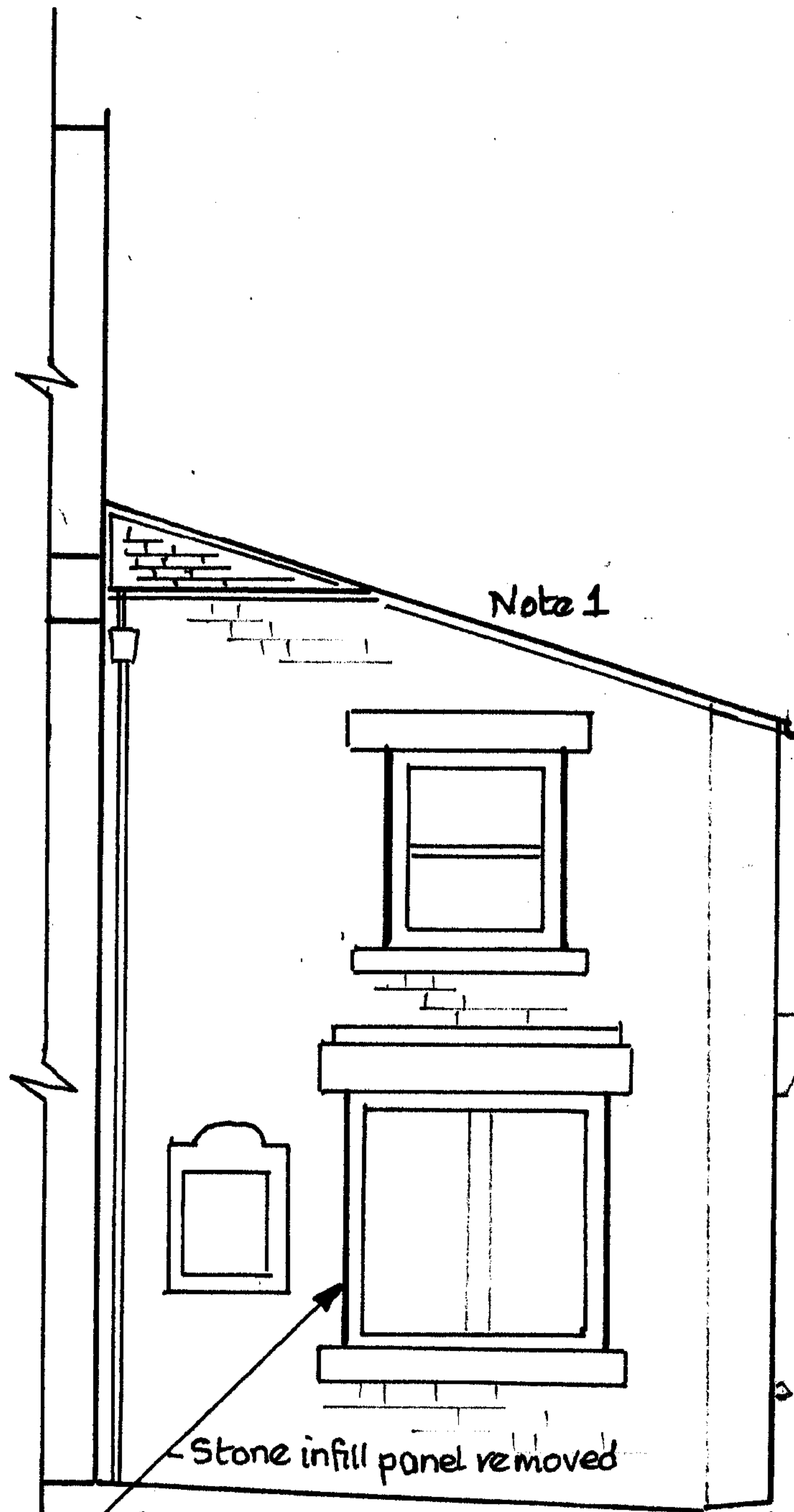
PROPOSED SW ELEVATION
