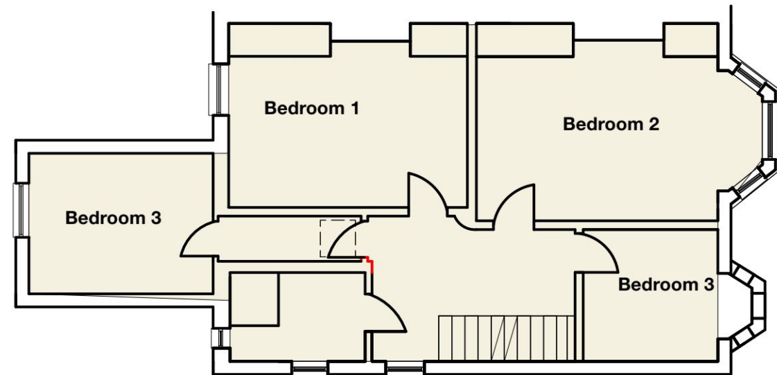
SECOND FLOOR PLAN 1:100@ A3
