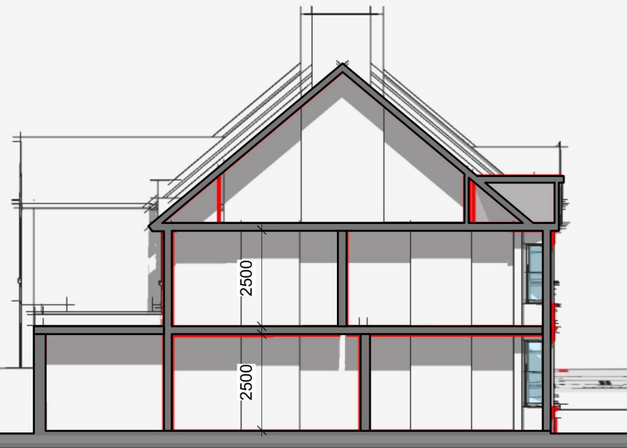
Cross Section 1:100 @A3
