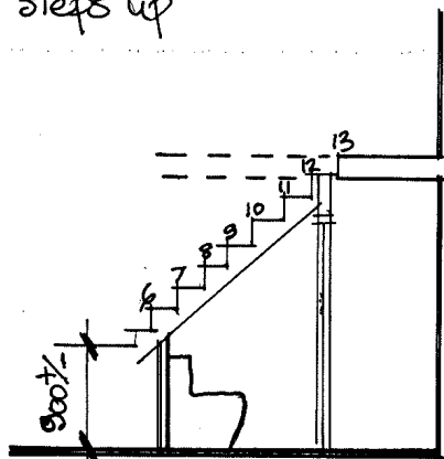
INDICATIVE SECTION (Ground Floor WC)
