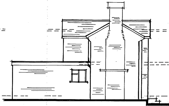
SIDE (North) ELEVATION (As Existing)
