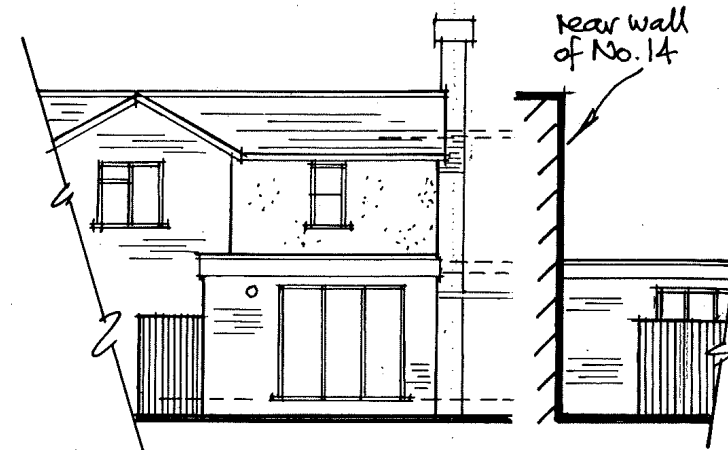
REAR (East) ELEVATION (As Existing)
