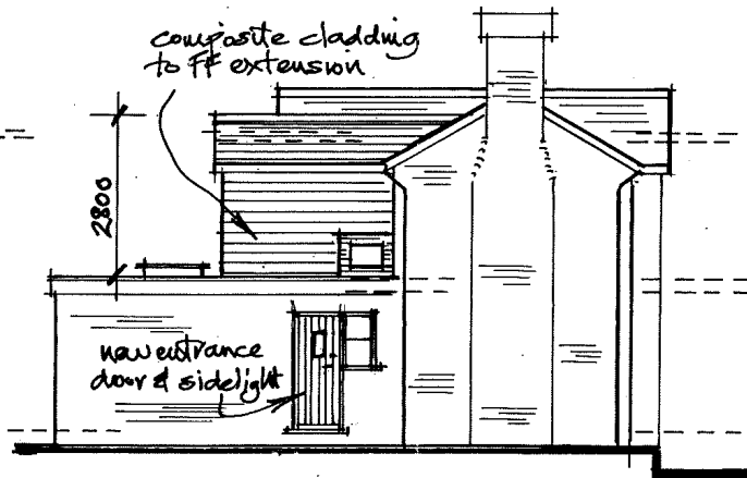
SIDE (North) ELEVATION (As Proposed)
