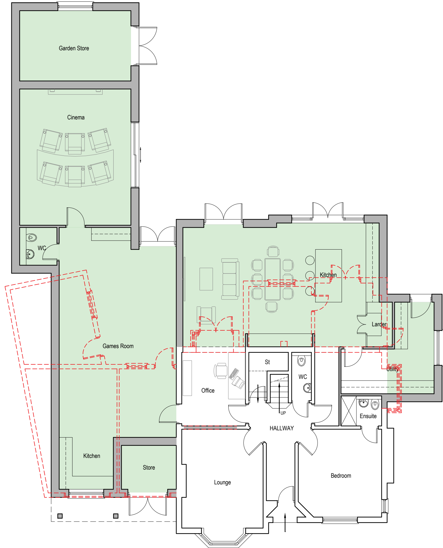
01 PROPOSED GROUND FLOOR PLAN Scale 1:100
