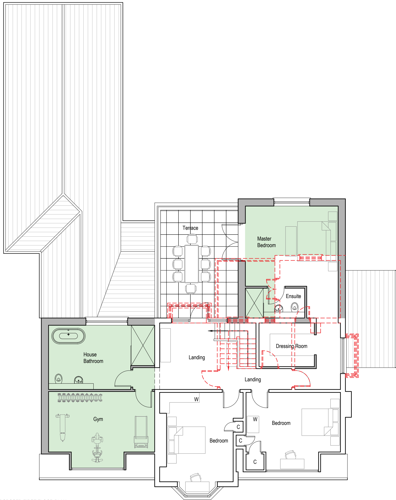
01 PROPOSED FIRST FLOOR PLAN Scale 1:100
