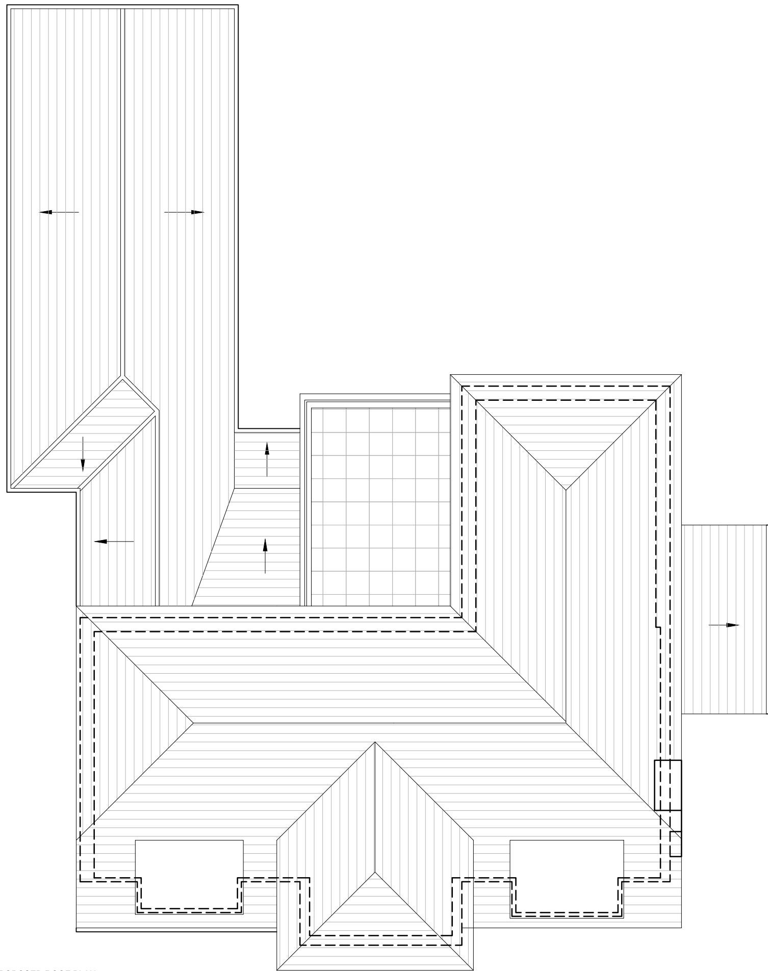
01 PROPOSED ROOF PLAN Scale 1:100
