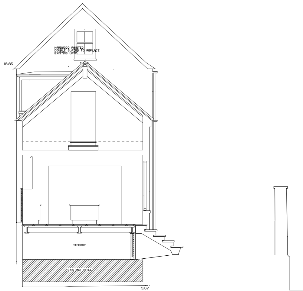
PART SECTION - PROPOSED, WEST.
