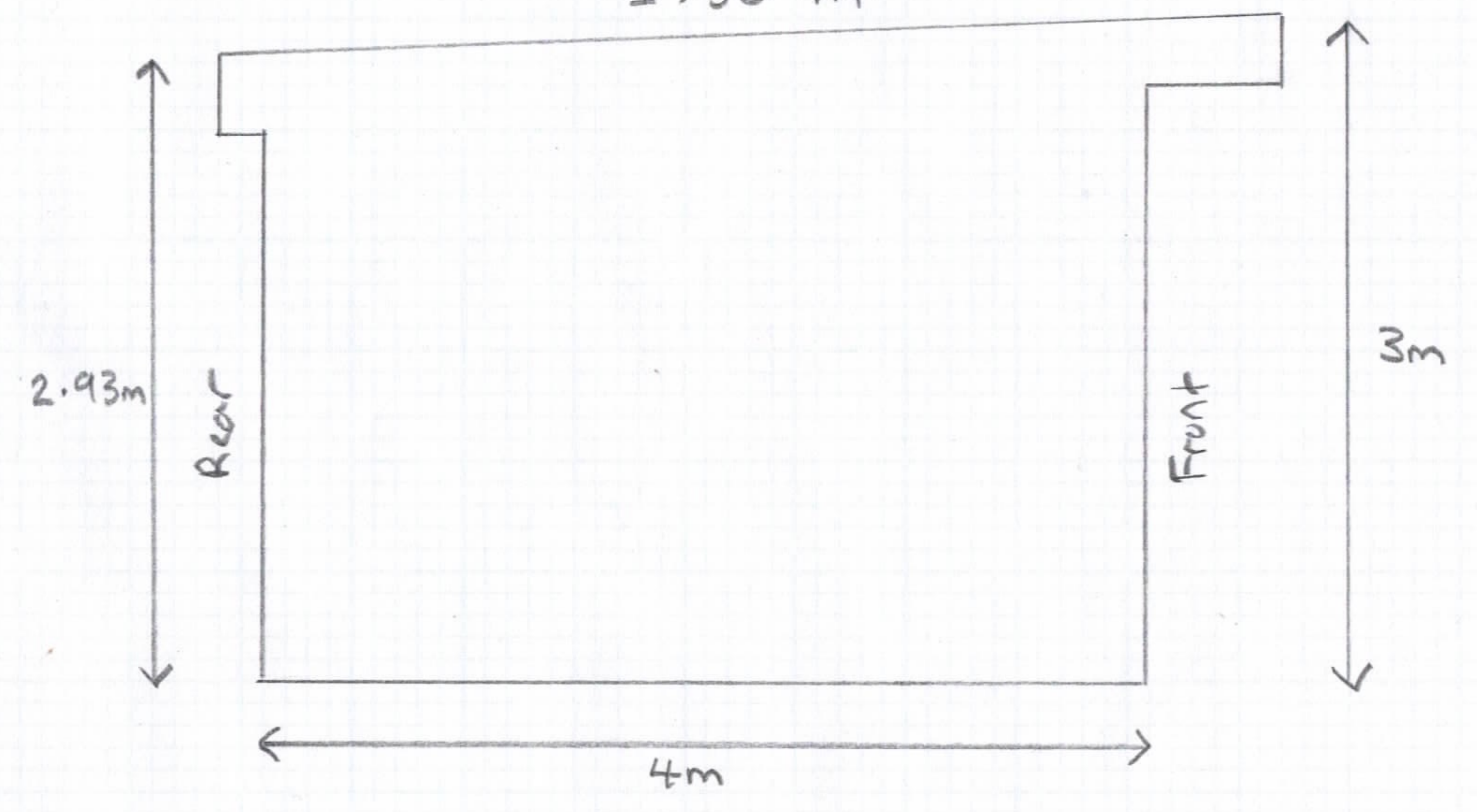
Proposed Side Elevation 1:50 A4
