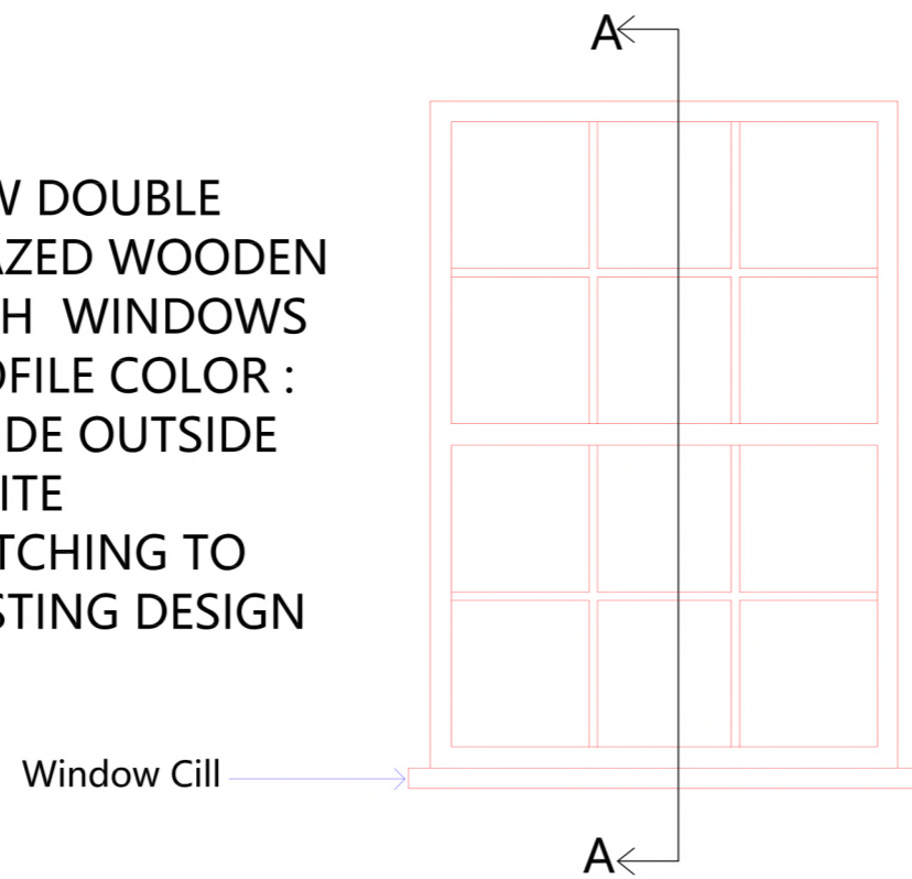
Window Elevation
