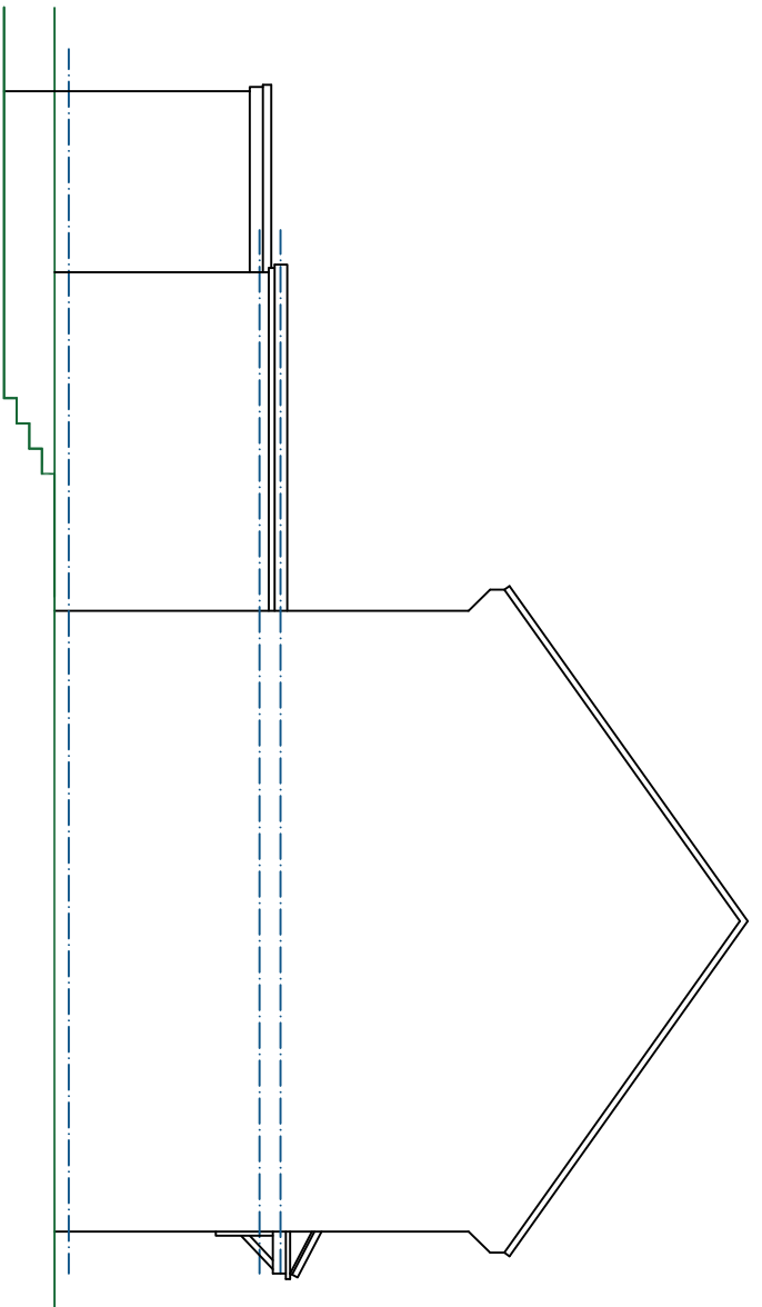
Side Elevation (Party Wall)
