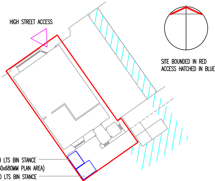
BLOCK PLAN SCALE 1:200
