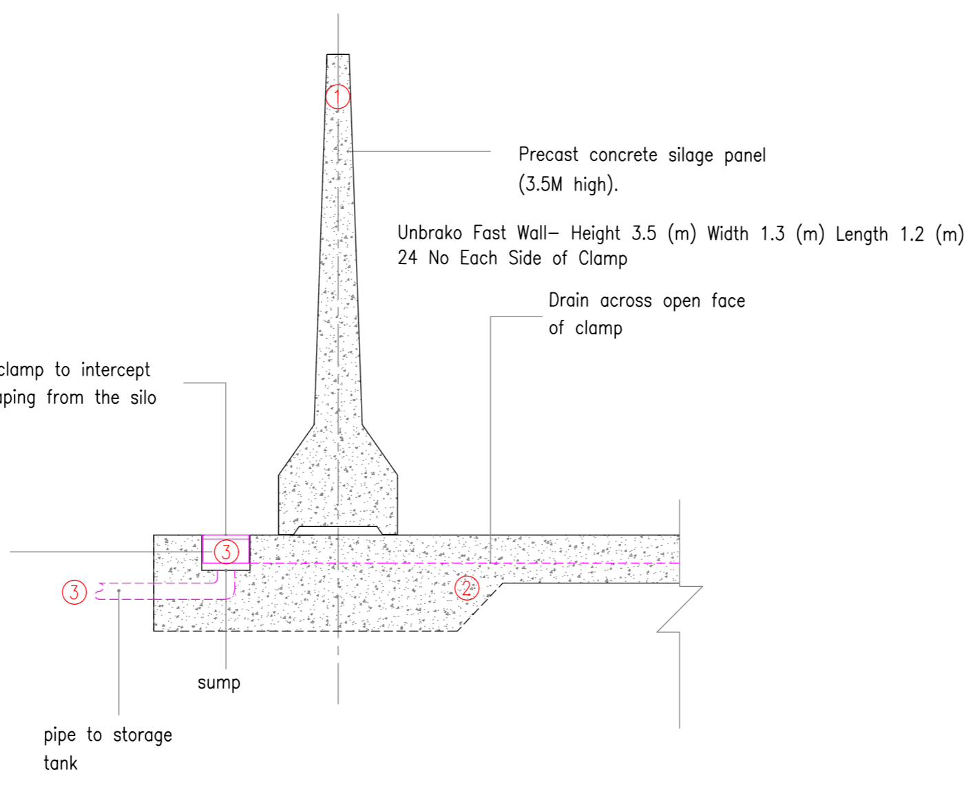
Example of External Boundary Channel (not to scale)
