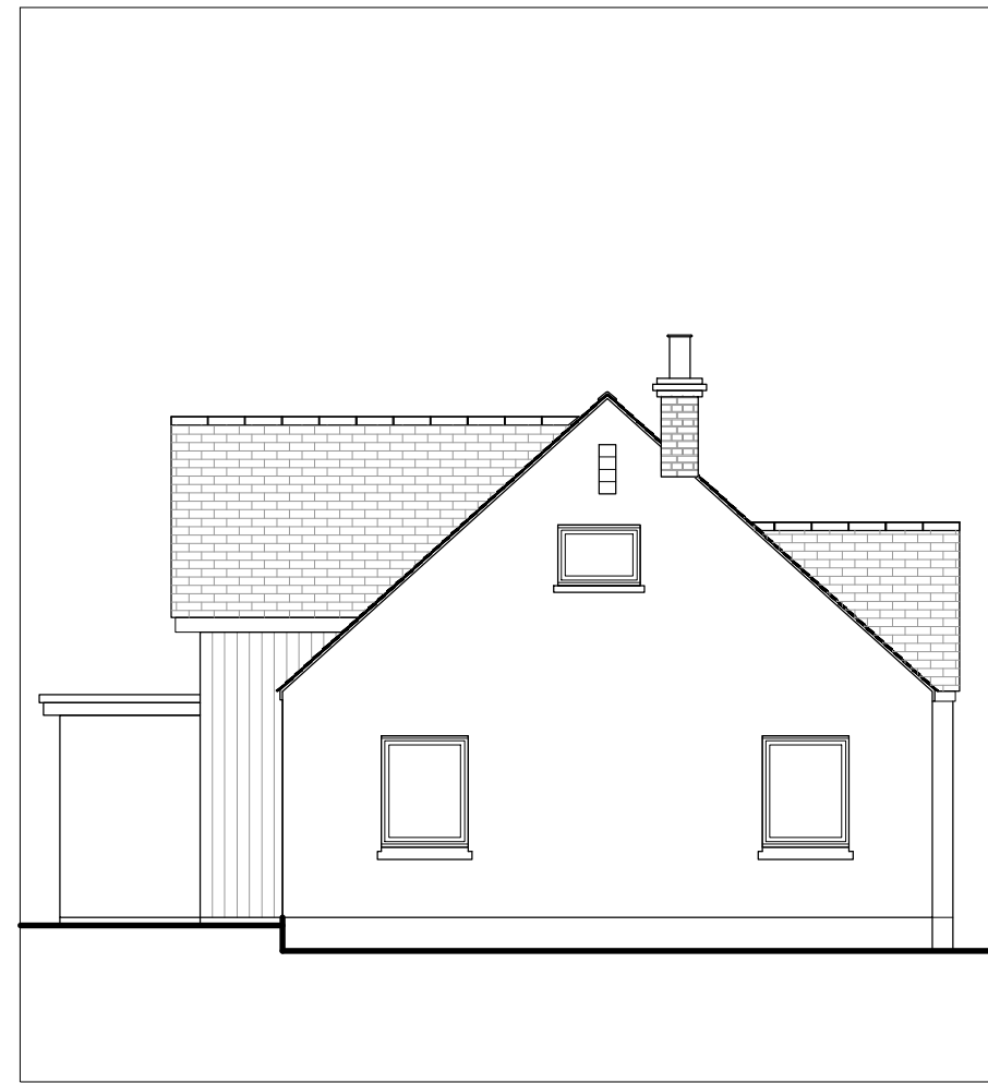
02 PROPOSED SOUTH ELEVATION 1:100
