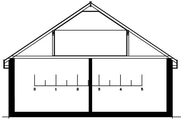
EXISTING CROSS SECTION
