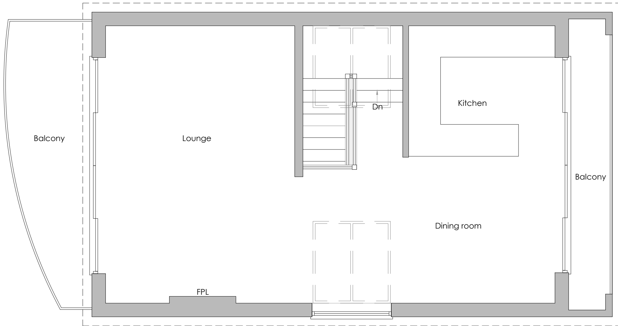
First Floor Plan As Proposed
