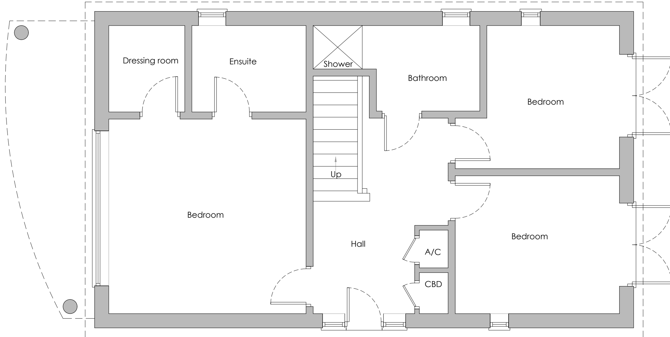
Ground Floor Plan As Proposed
