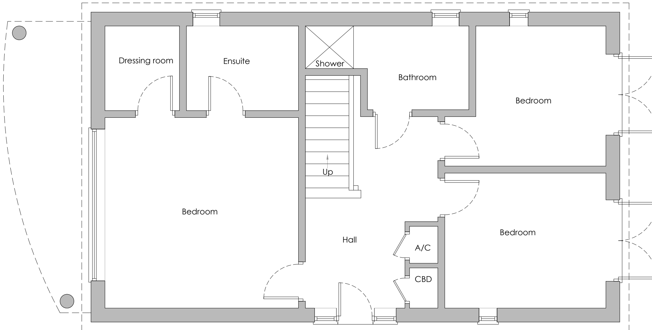
Ground Floor Plan As Existing
