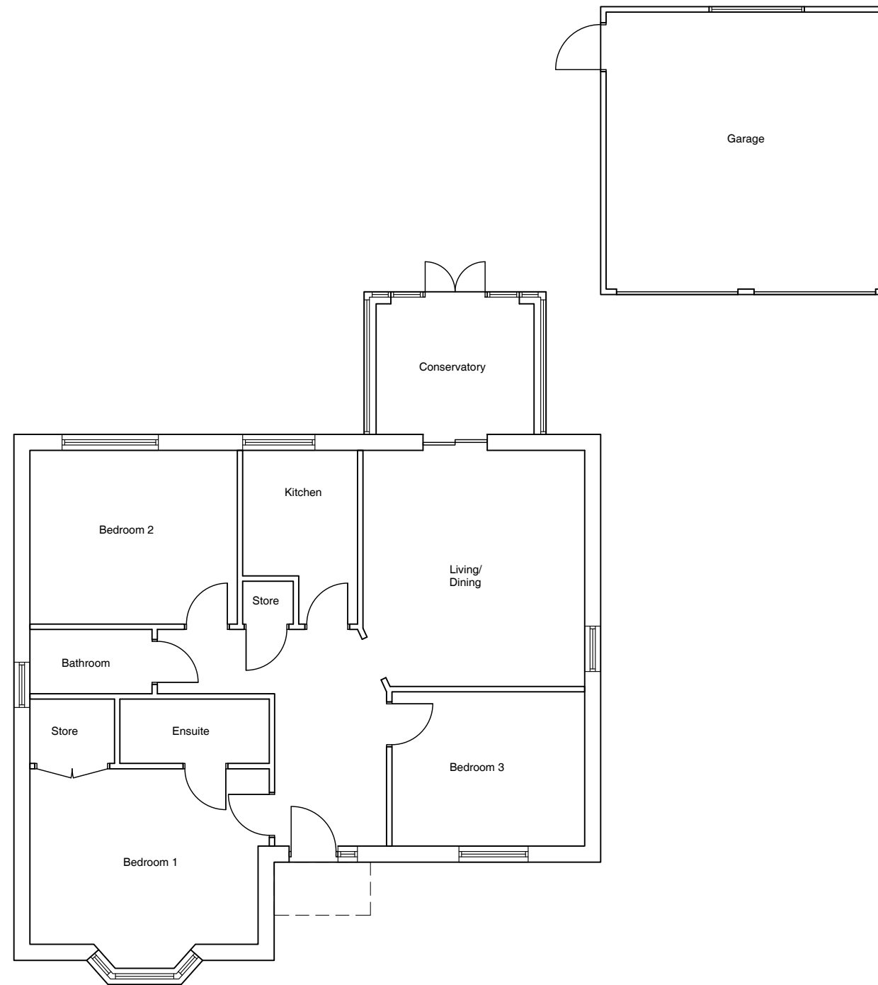
EXISTING GROUND FLOOR PLAN SCALE 1:100@A3
