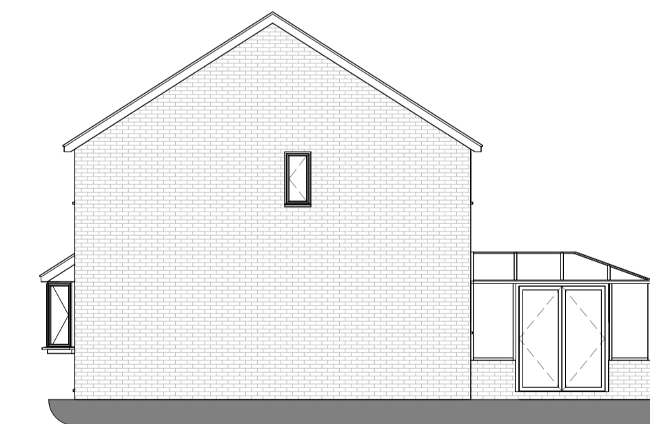
8 Existing East Elevation 1:100
