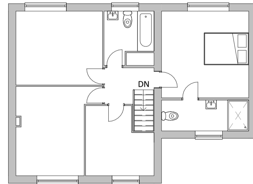
4 Proposed First Floor Plan 1:100
