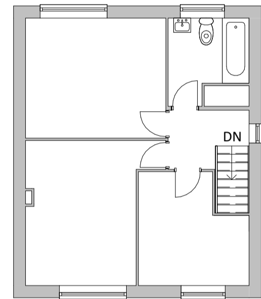
3 Existing First Floor Plan 1:100
