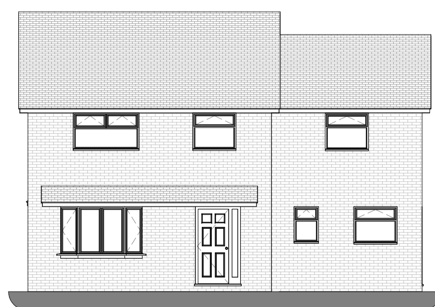
9 Proposed South Elevation 1:100
