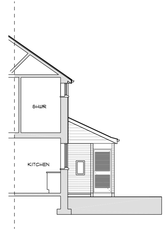
EXISTING SIDE ELEVATION - SOUTH EAST Scale 1:100 @ A3
