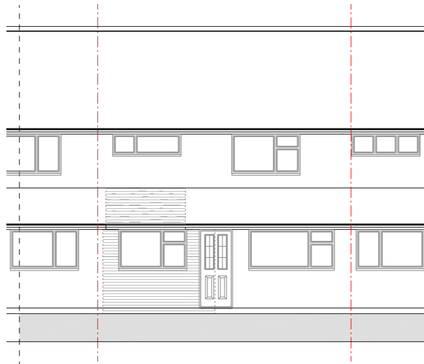
PROPOSED FRONT ELEVATION - NORTH EAST Scale 1:100 @ A3
