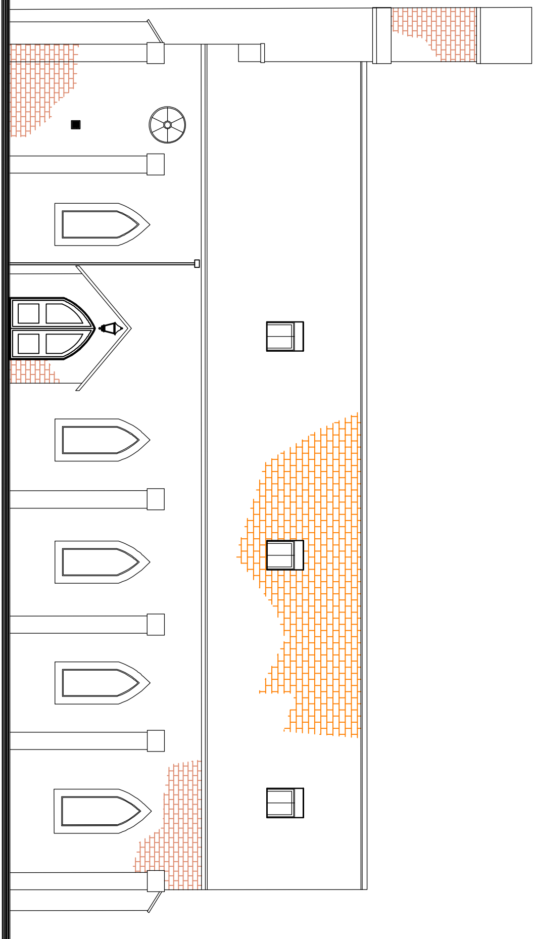
EXISTING SOUTH ELEVATION SCALE 1:100 @ A3
