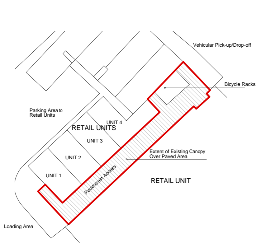
SITE PLAN (Existing) 1:500
