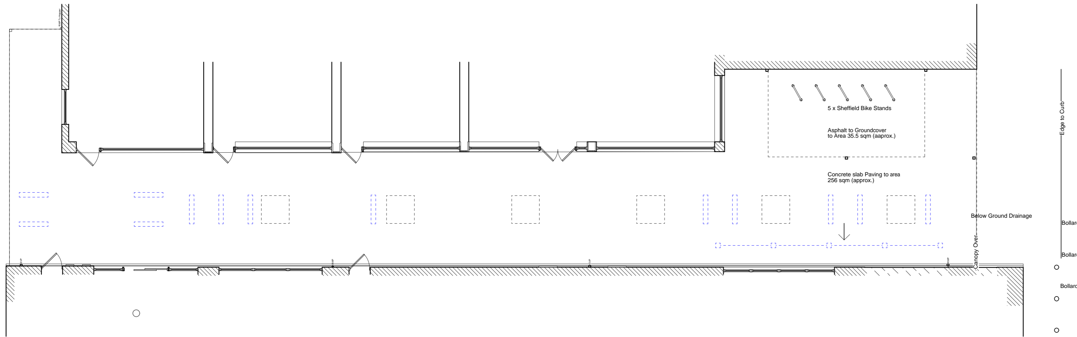
GROUND FLOOR/CANOPY PLAN (Existing) 1:100
