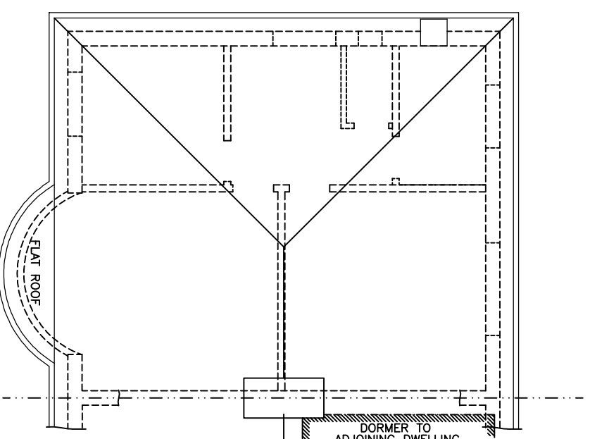
ROOF PLAN (1:100)
