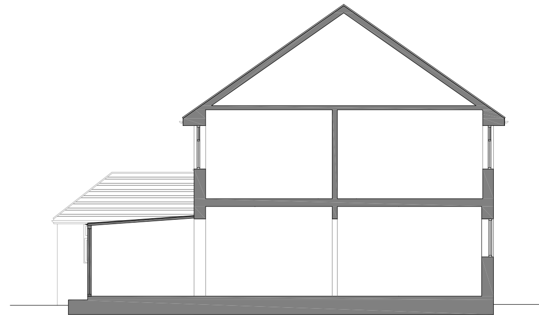
Existing A-A SECTION
