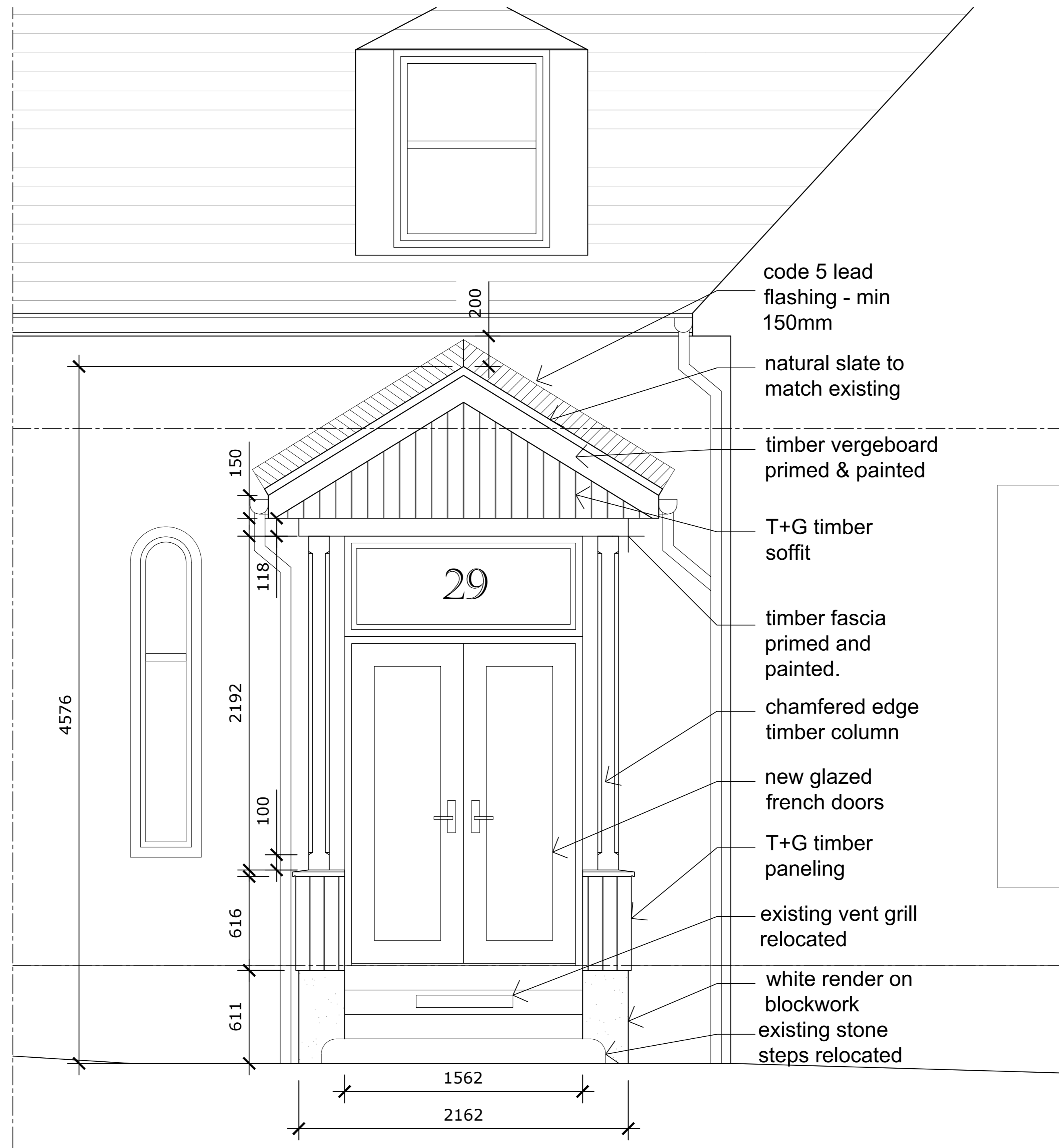
Porch Elevation as Proposed, 1:20
