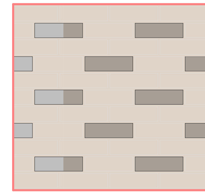
BRICK FINISH 04 - Textured Brickwork 1:10
