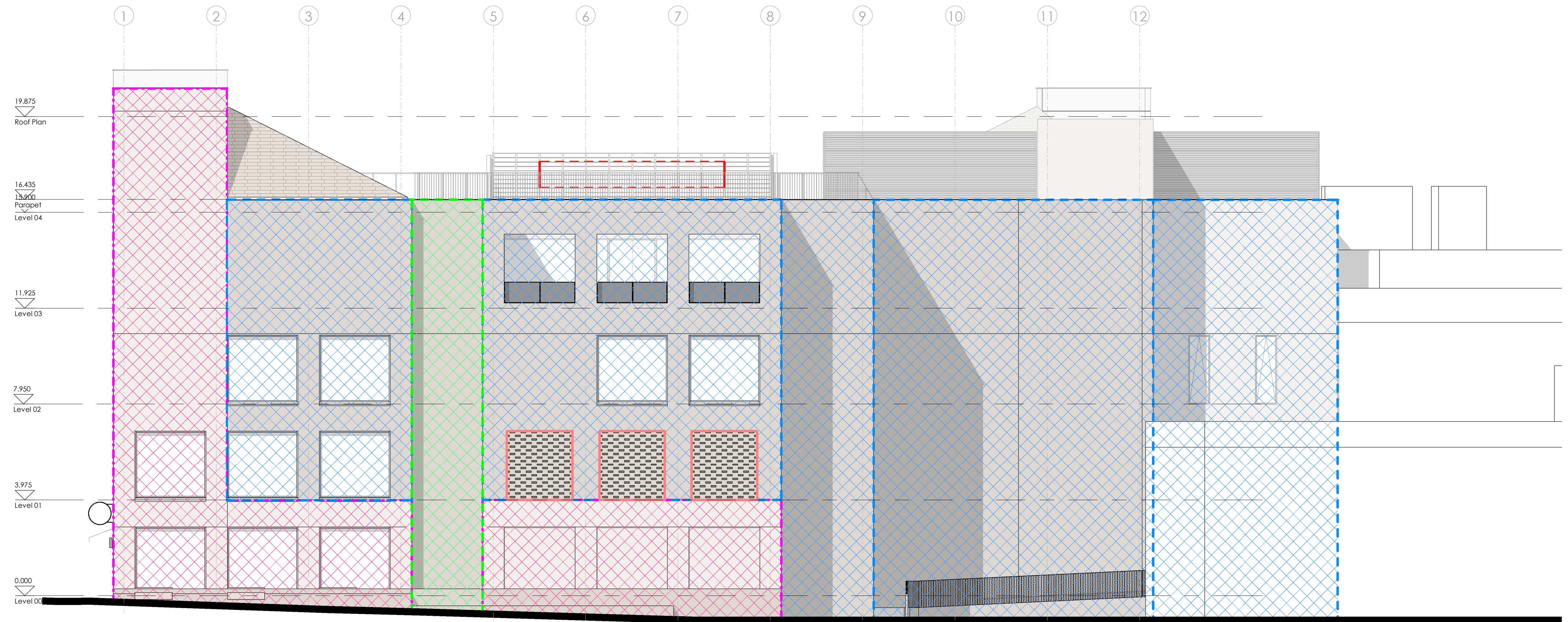
South Elevation MATERIALITY 1:100
