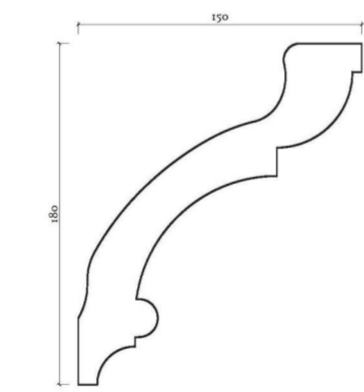
Proposed Georgian cornices
