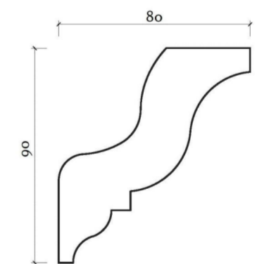
Proposed Georgian cornices
