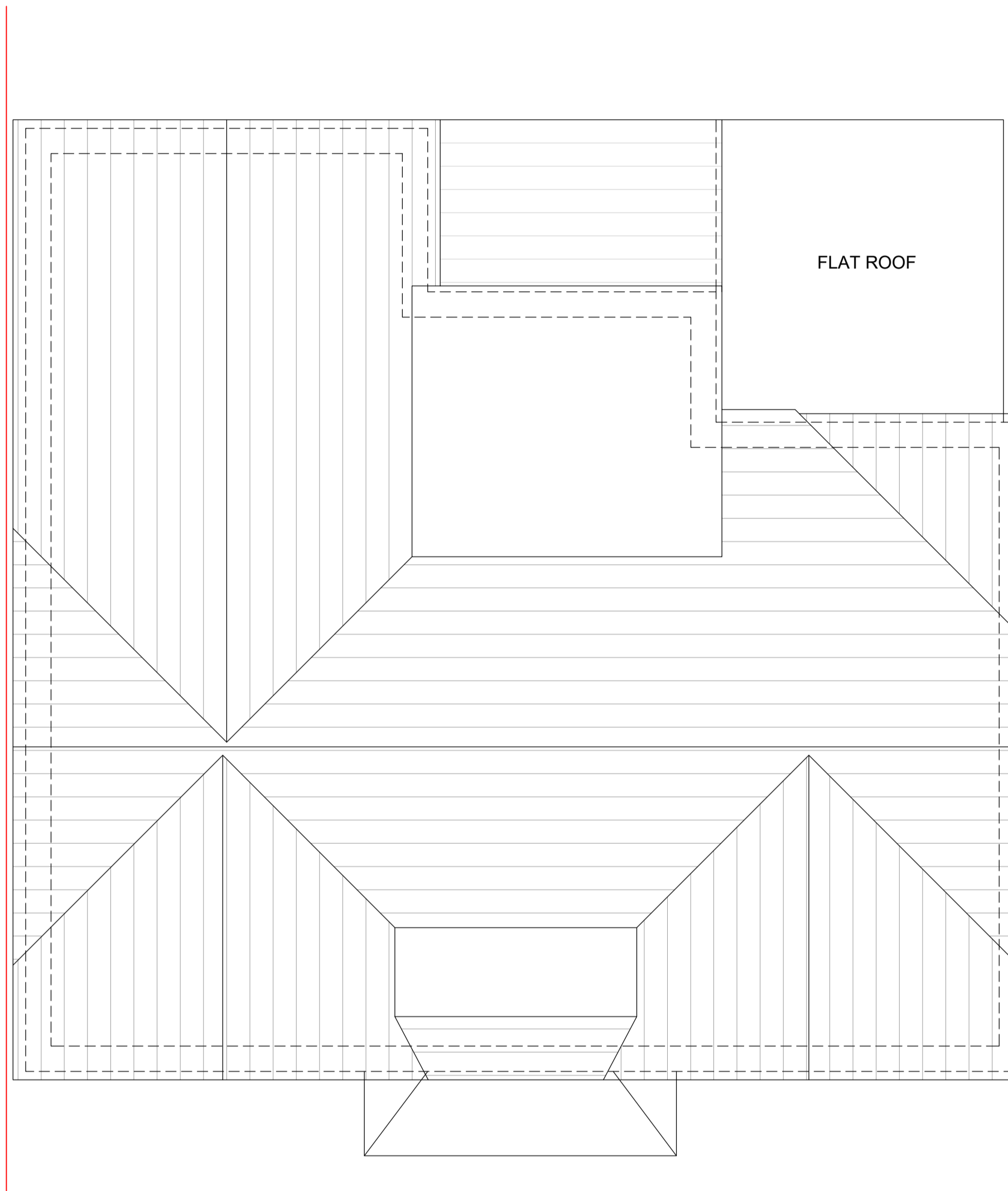
ROOF PLAN
