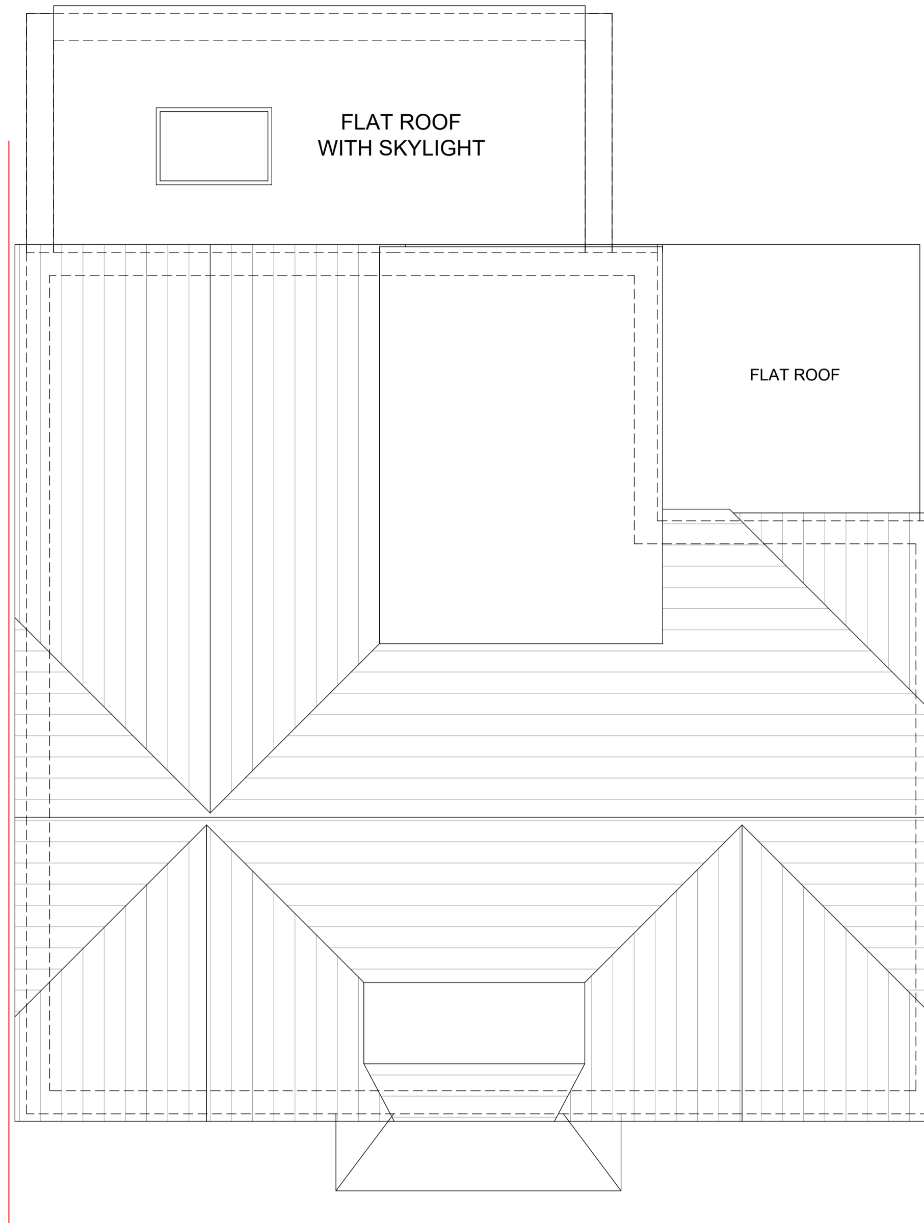
ROOF PLAN
