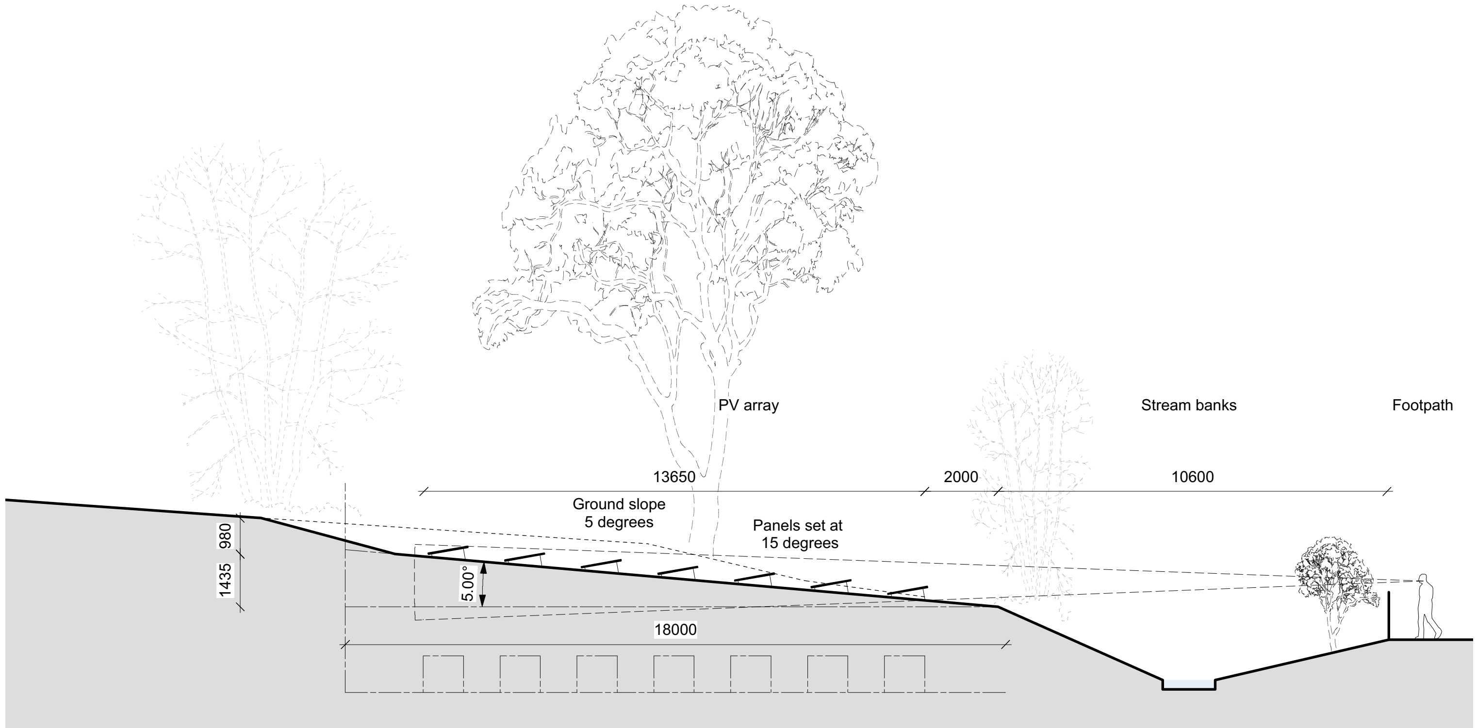
1 Proposed site section Scale: 1:100
