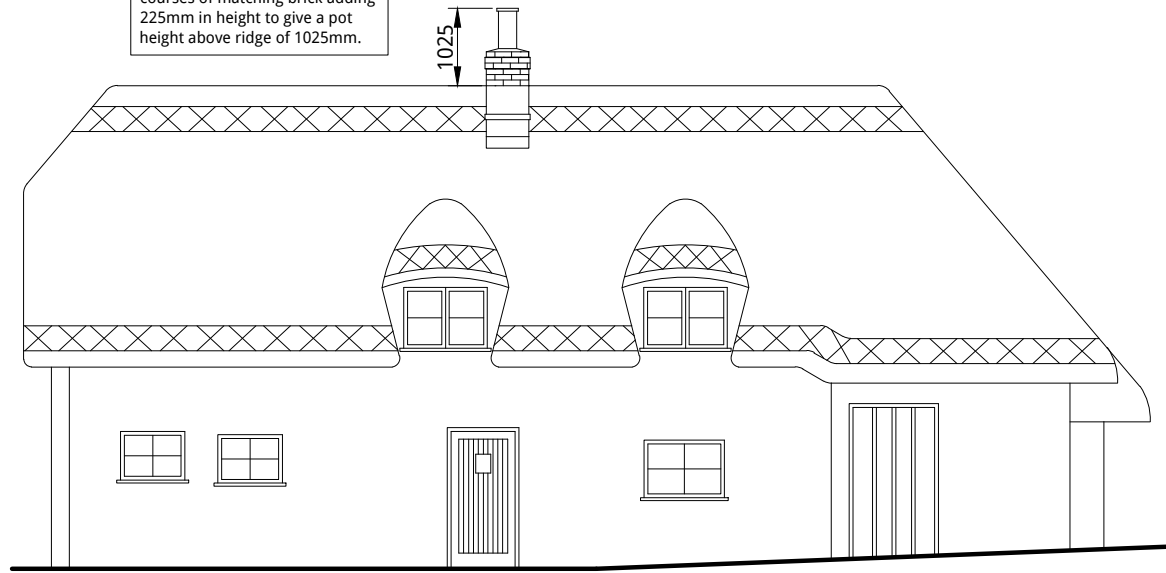
PROPOSED FRONT (EAST) ELEVATION
