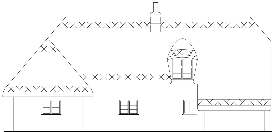
EXISTING REAR (WEST) ELEVATION
