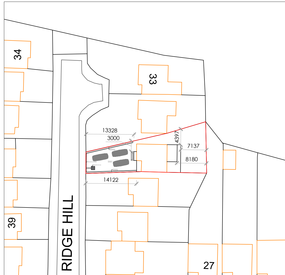
Block Plan @ 1:500
