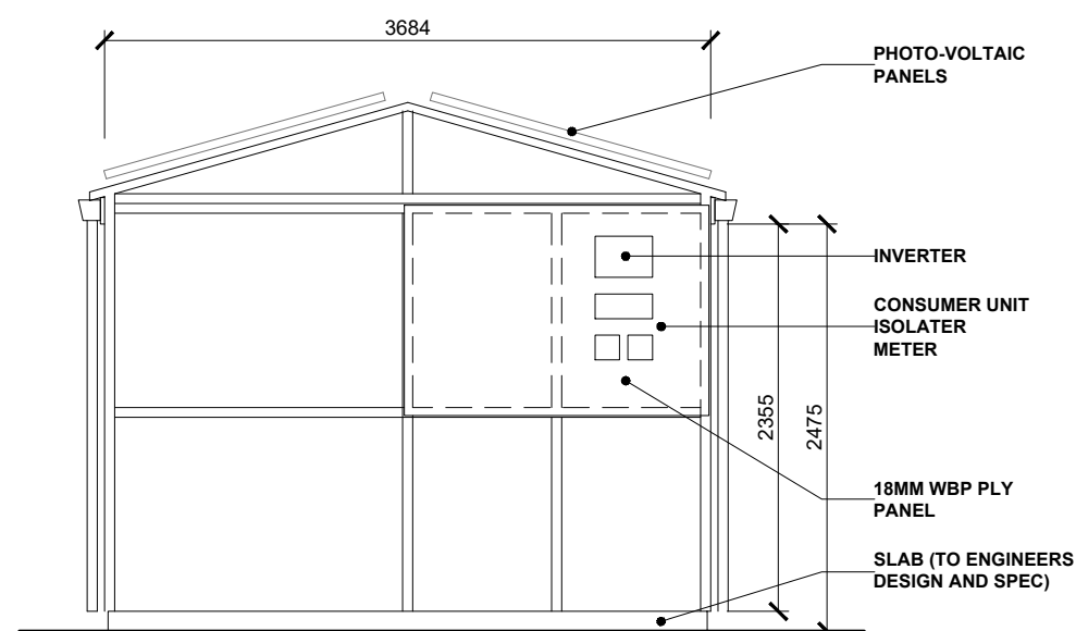
GARAGE SECTION
