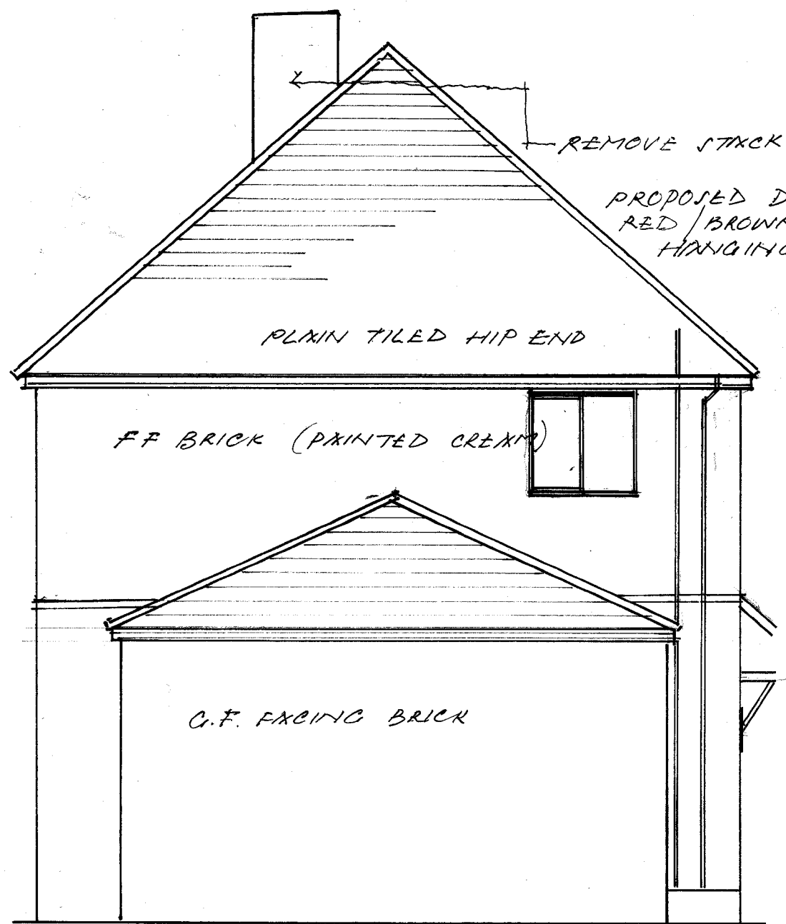
EXISTING S.E. ELEVATION
