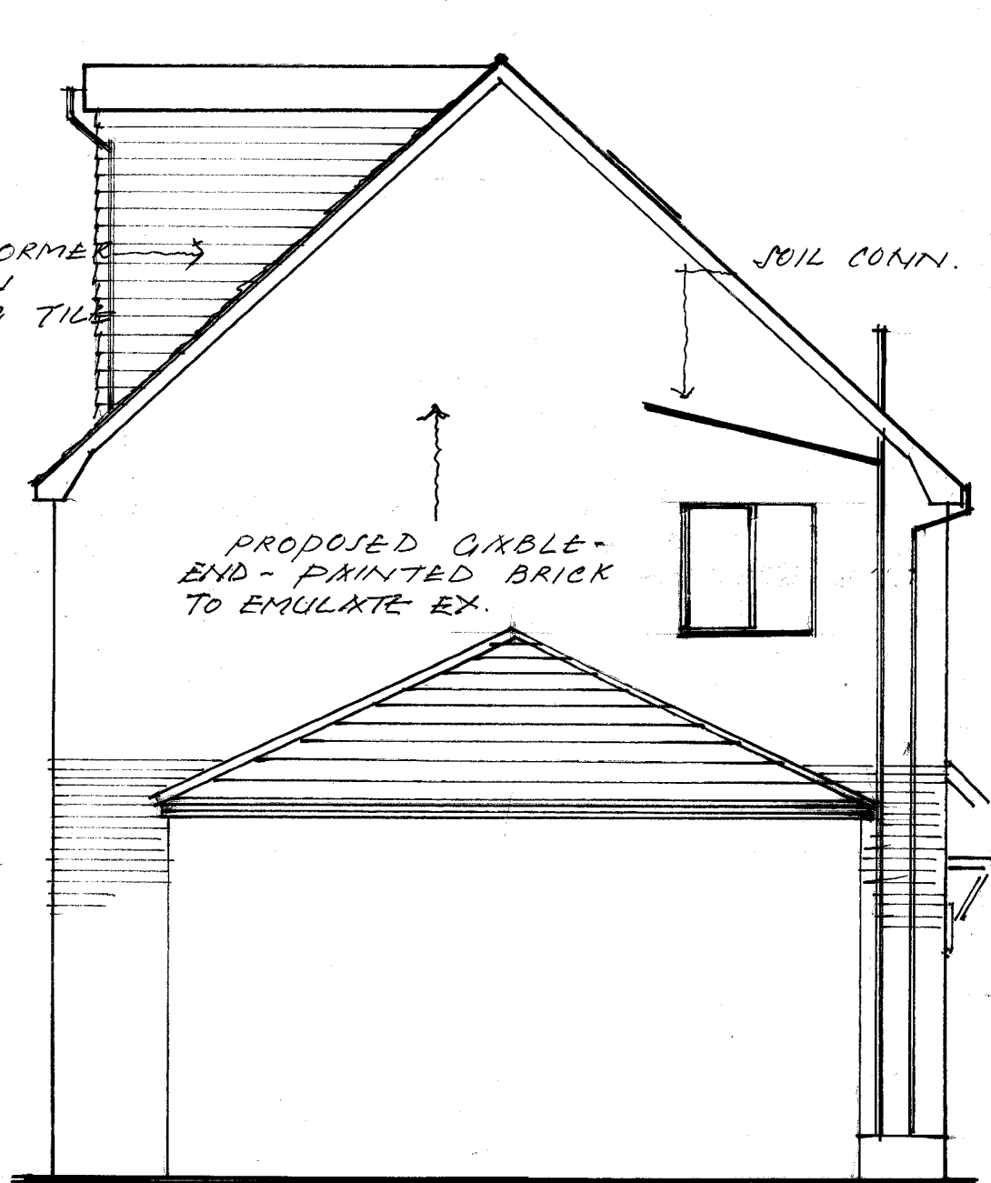
PROPOSED S.E. ELEVATION
