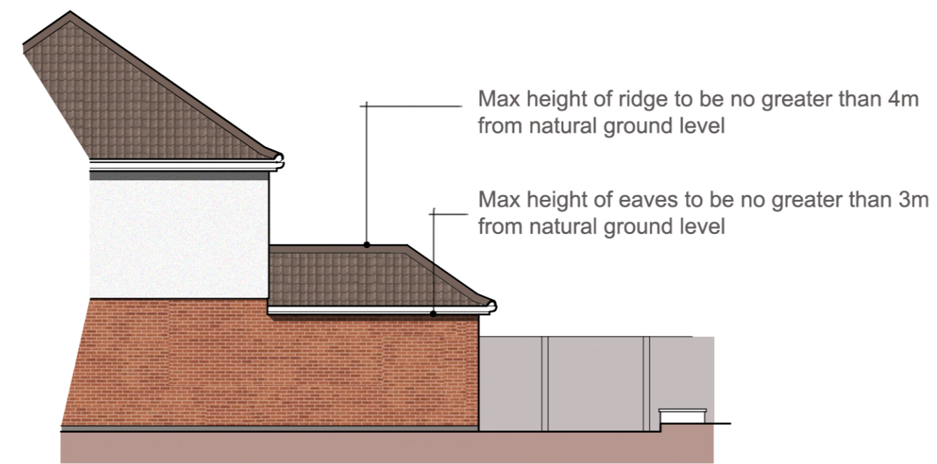
Proposed (Side) North Elevation Scale 1:100
