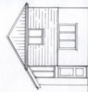
East Elevation
