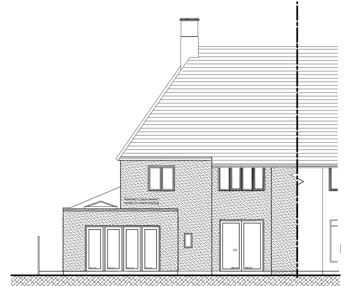
PROPOSED EAST (REAR) ELEVATION
