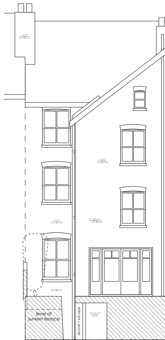
Rear East - Proposed
