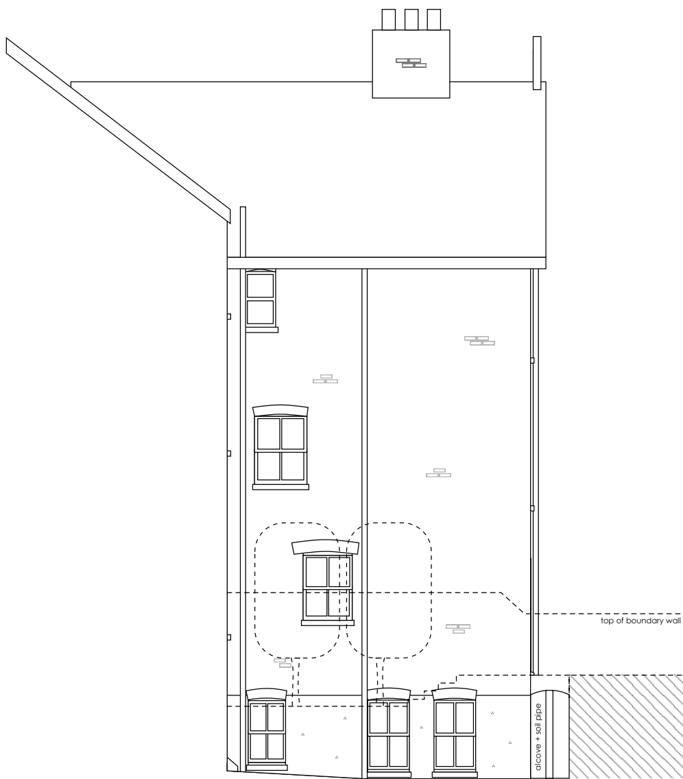
Rear South - Proposed
