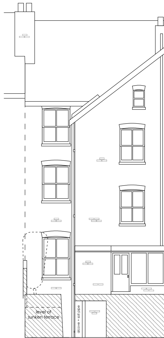
Rear East - Existing
