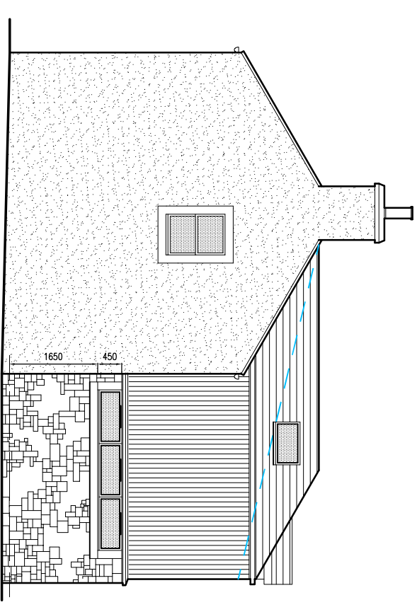
PROPOSED SIDE (SE) ELEVATION 1 : 100 @ A3
