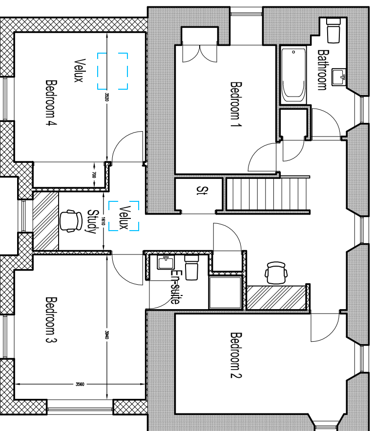
PROPOSED UPPER FLOOR PLAN 1 : 100 @ A3
