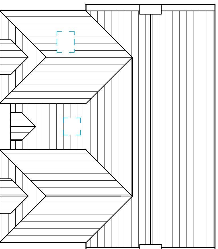
PROPOSED ROOF PLAN 1 : 100 @ A3
