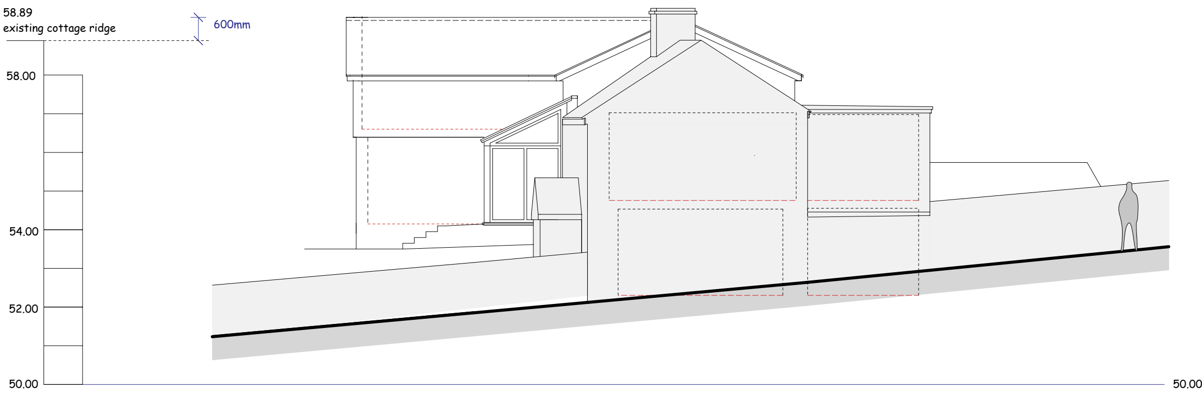
Proposed South-East Elevation.
