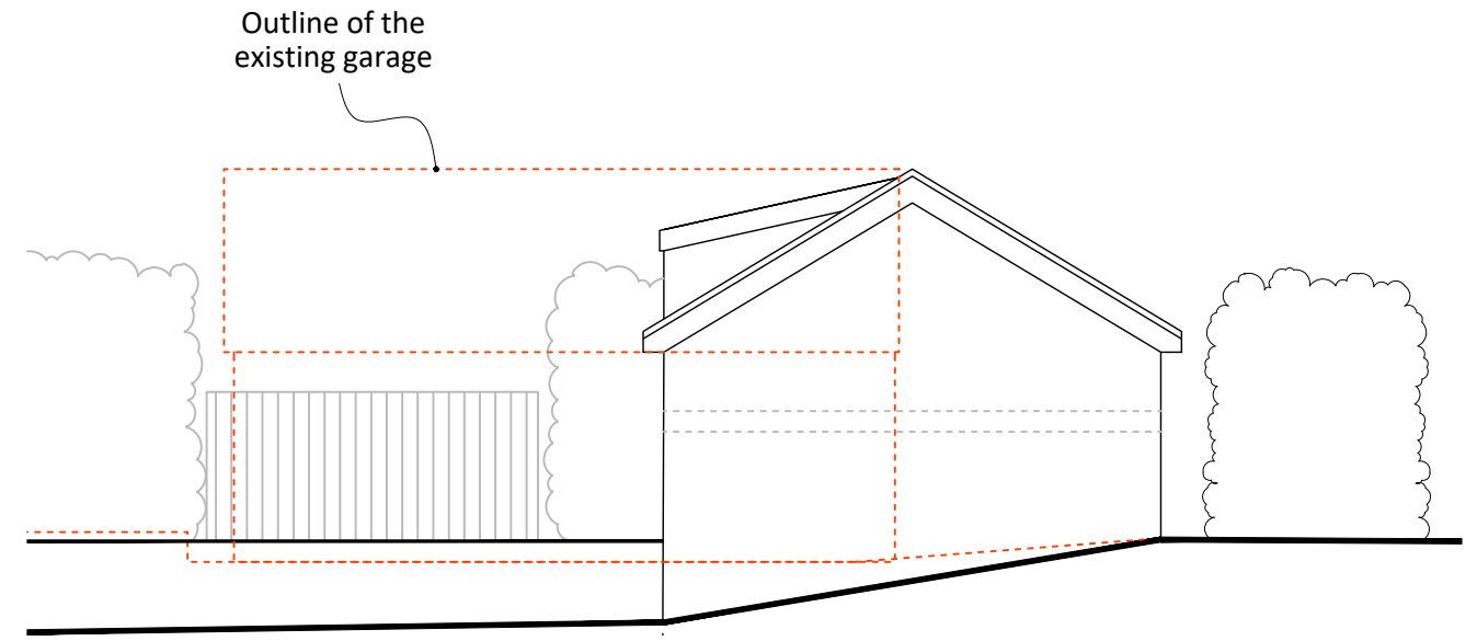
Side Elevation (North West)
