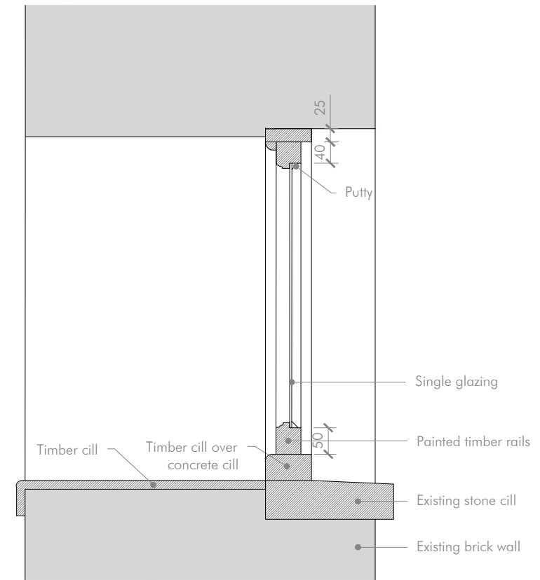
Sectional View - Window Head and Cill
